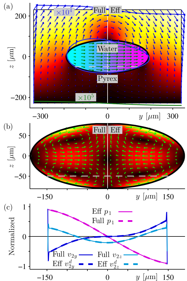
FIG. 5. (Color online) Full (left) and effective (right) simulations for a curved channel with fluid-solid coupling. (a) An elliptical fluid domain with the acoustic pressure p_1 from -0.35 \text{ MPa} (dark purple) to +0.35 \text{ MPa} (light cyan) and fluid velocity (green arrows, max 0.2 \text{ m/s} ) surrounded by solid Pyrex with a displacement field u_{sl} (dark blue arrows) and displacement magnitude |u_{sl}| from 0 \text{ nm} (black) to 2.7 \text{ nm} (yellow). To be visible, the displacement (dark blue line and dark blue arrows, max 2.7 \text{ nm} ) is enhanced 10^4 times, except at the bottom (green line, max 0.1 \text{ nm} ) where it is enhanced 10^5 times. (b) Streaming velocity v_2 (light green arrows) and magnitude from 0 \mu\text{m/s} (black) to 7.8 \mu\text{m/s} (light yellow). (c) Line plots along the light ray dashed line in (a) and (b) of p_1 normalized by 0.35 \text{ MPa} and v_2 by 7.8 \mu\text{m/s} .
