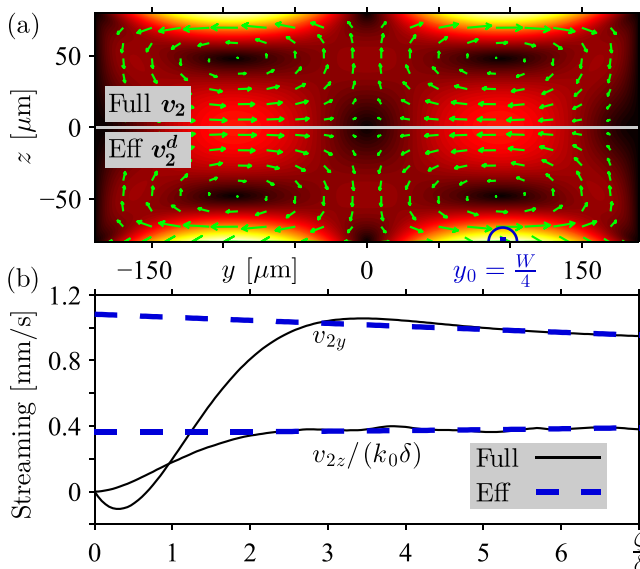
FIG. 4. (Color online) Simulated second-order velocity for the rectangular channel. (a) The full-model v_2 (above) and the effective-model v_2^d (below). (b) Line plots near the center of the dark blue half circle in (a) at y_0 = \frac{1}{4}W for -\frac{1}{2}H < z < -\frac{1}{2}H + 7\delta .
